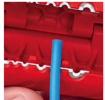
90 22 02 SB: Practical locator simplifies the insertion of single conductors for stripping
